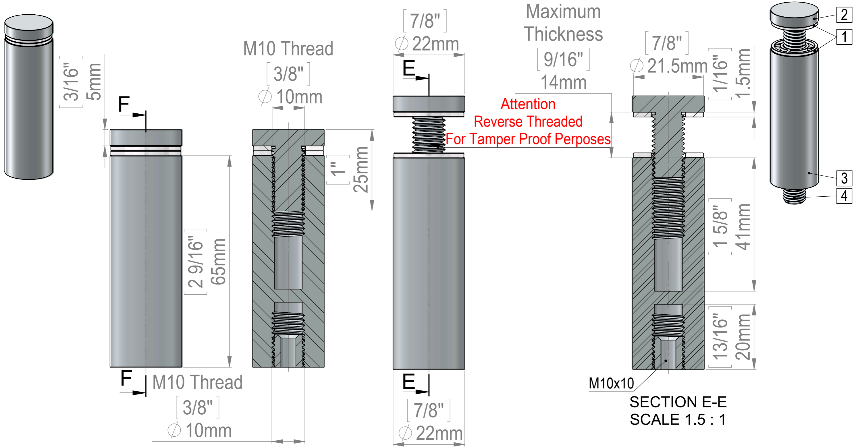
SECTION F-F SCALE 1.5 : 1
