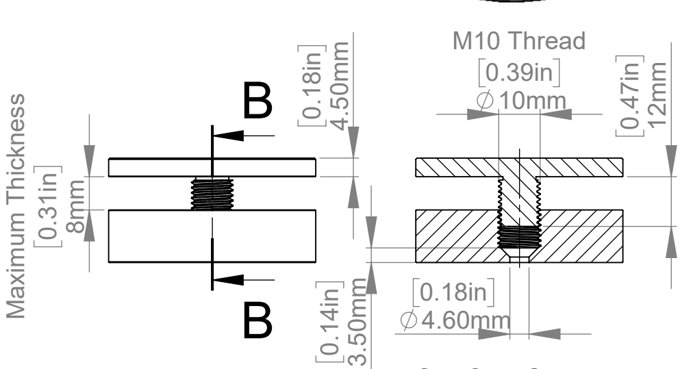
SECTION B-B SCALE 1 : 1.25
